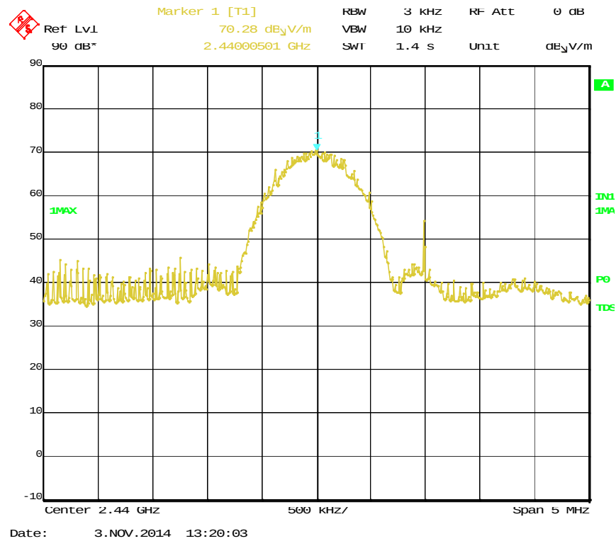
Figure 26 — 2440 MHz
