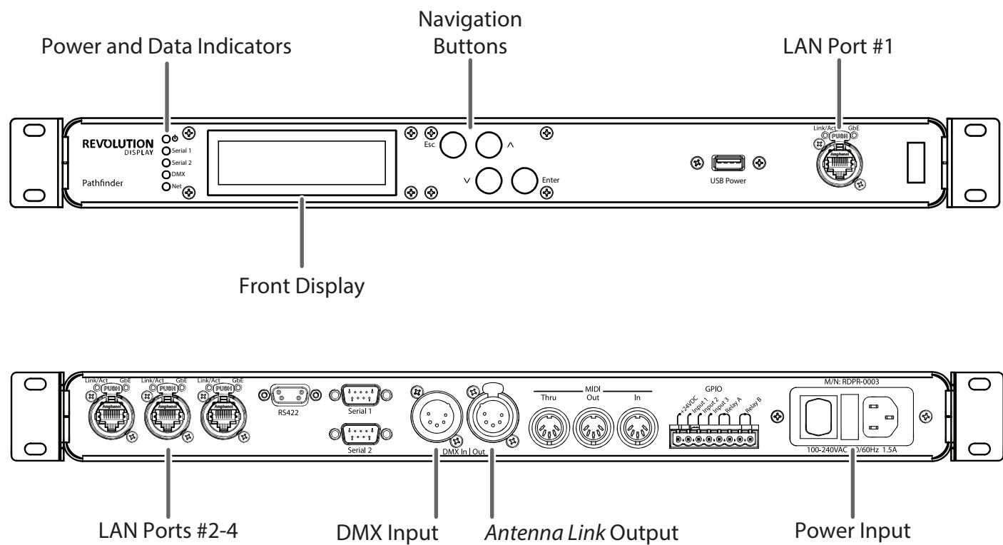
Figure 6. Pathfinder components.
