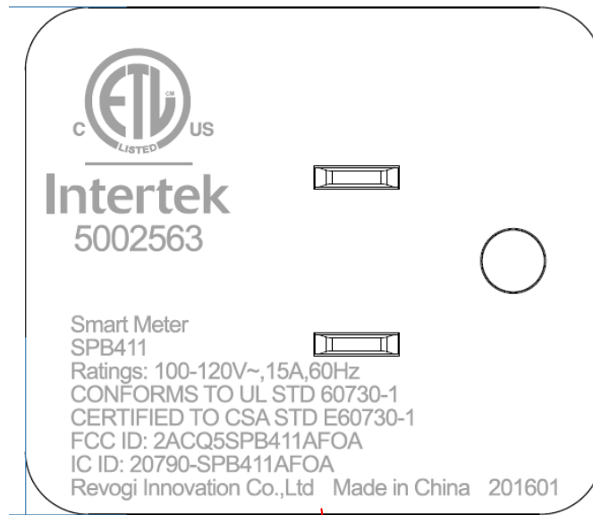
Proposed Label Location on EUT EUT Back View/ proposed Label Location
