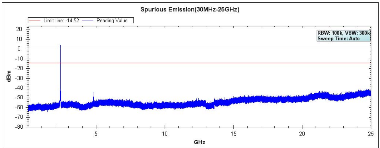
Channel 01 (2412MHz)
