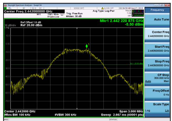
2442MHz,Plot 1,Reference Level
