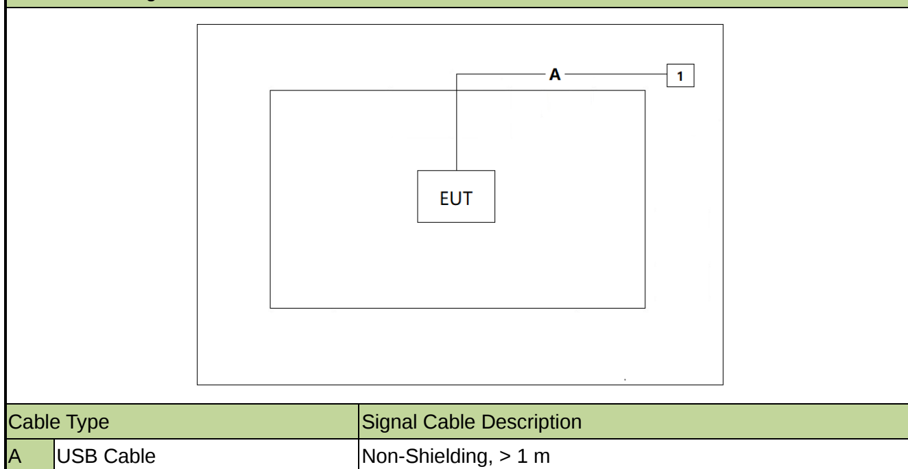
Connection Diagram for Radiated Emissions Measurement
