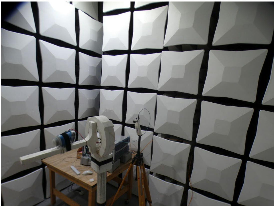
Photo 6: Test setup for radiated measurements above 26 GHz
