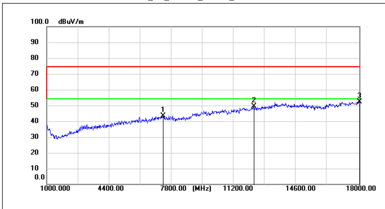
TX_CH_2479.28_Veritical_Peak
