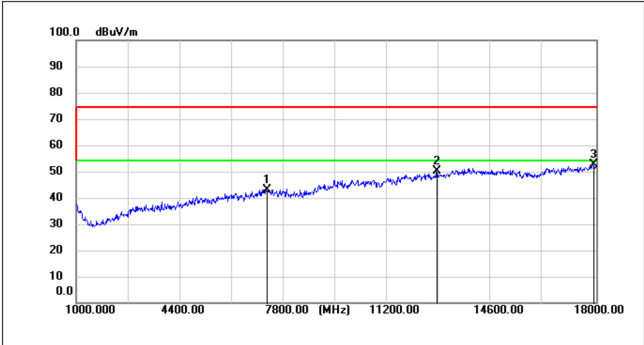
TX_CH_2479.28_Horizontal_Peak
