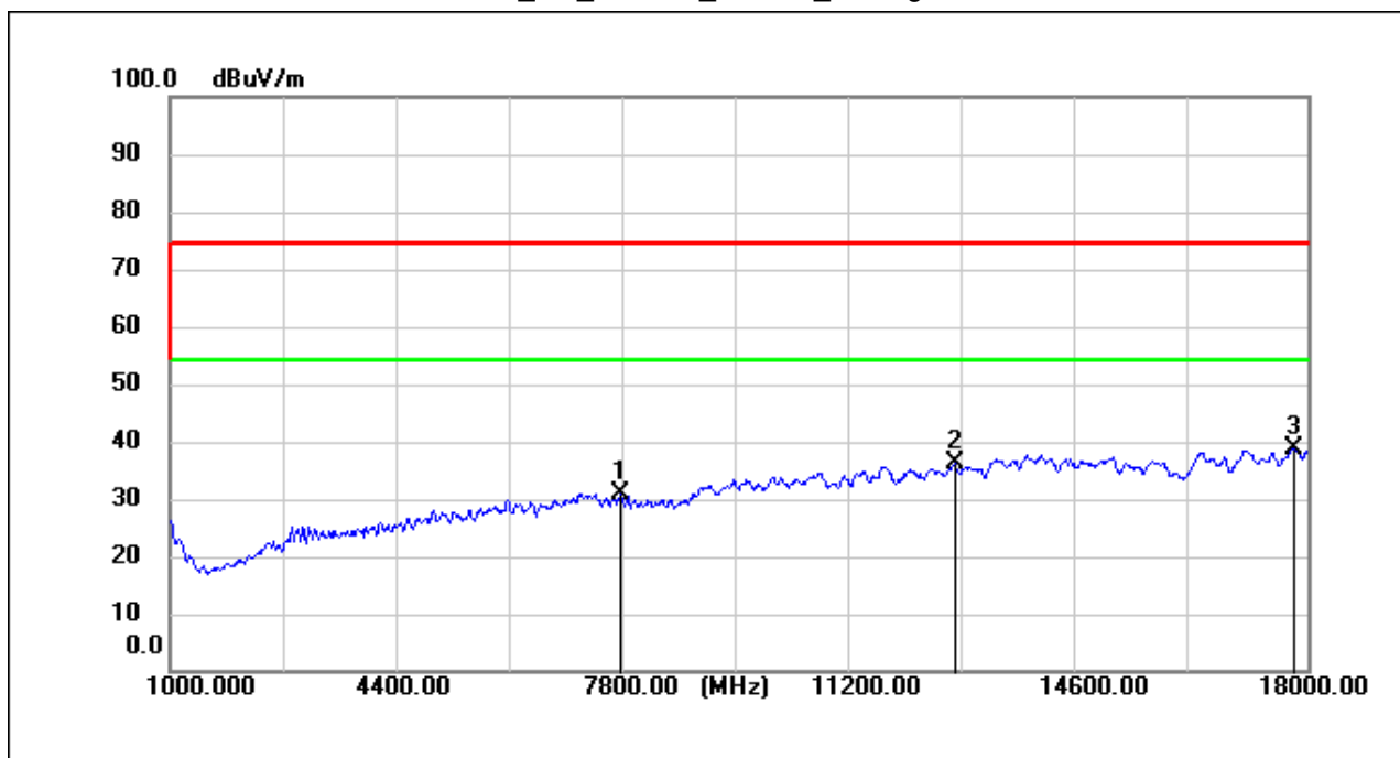
TX_CH_2479.28_Veritical_Average
