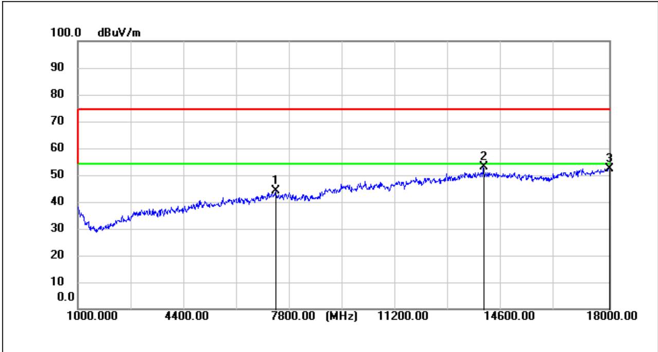
TX_CH_2441.84_Horizontal_Peak
