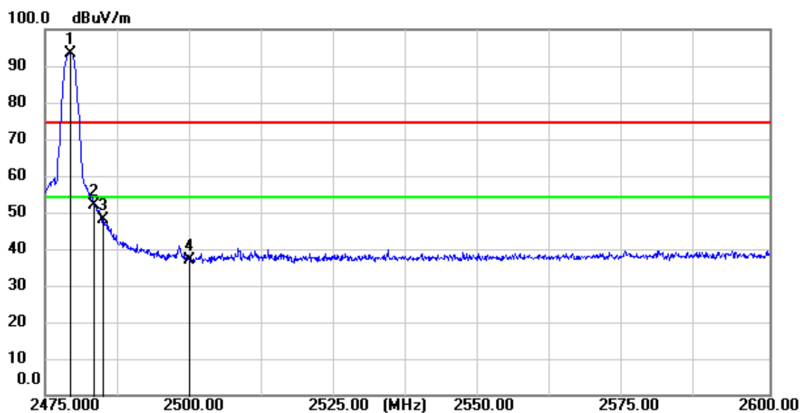
TX_CH_2479.28_Horizontal_Peak
