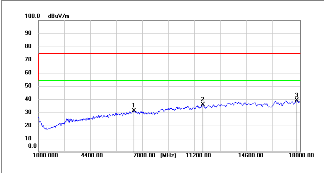
TX_CH_2404.06_Veritical_Average
