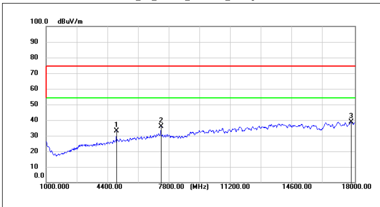
TX_CH_2441.84_Horizontal_Average
