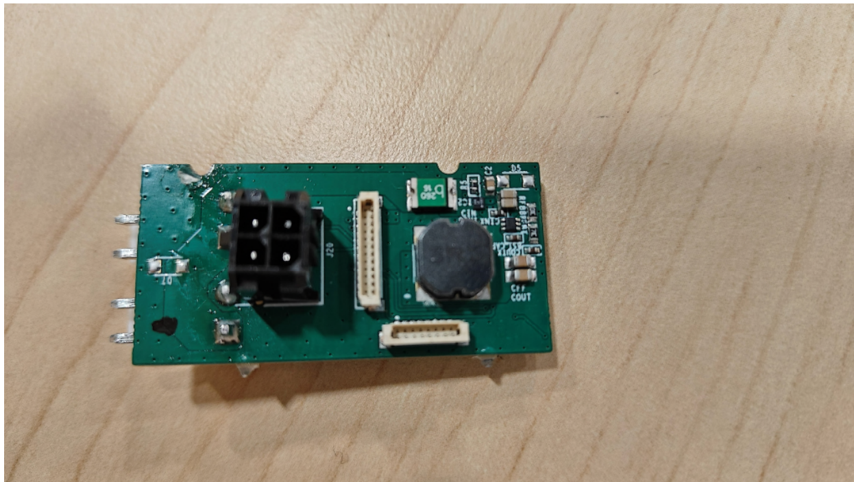
Figure 7 – Power PCB, Top
