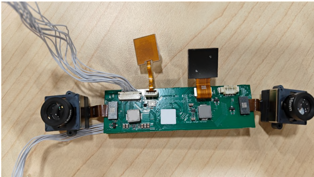
Figure 9 – Main PCB, Top
