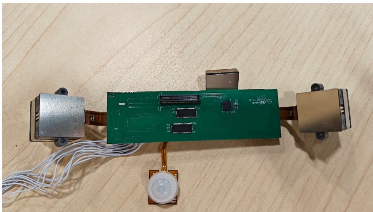
Figure 10 – Main PCB, Bottom
