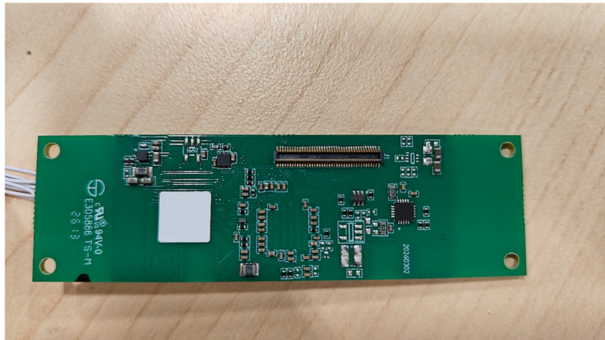
Figure 12 – Daughter PCB, Bottom
