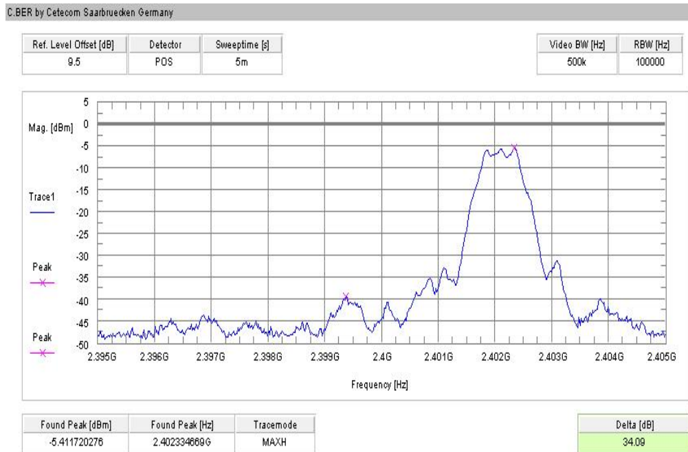
Plot 3: Lower band edge – hopping off
