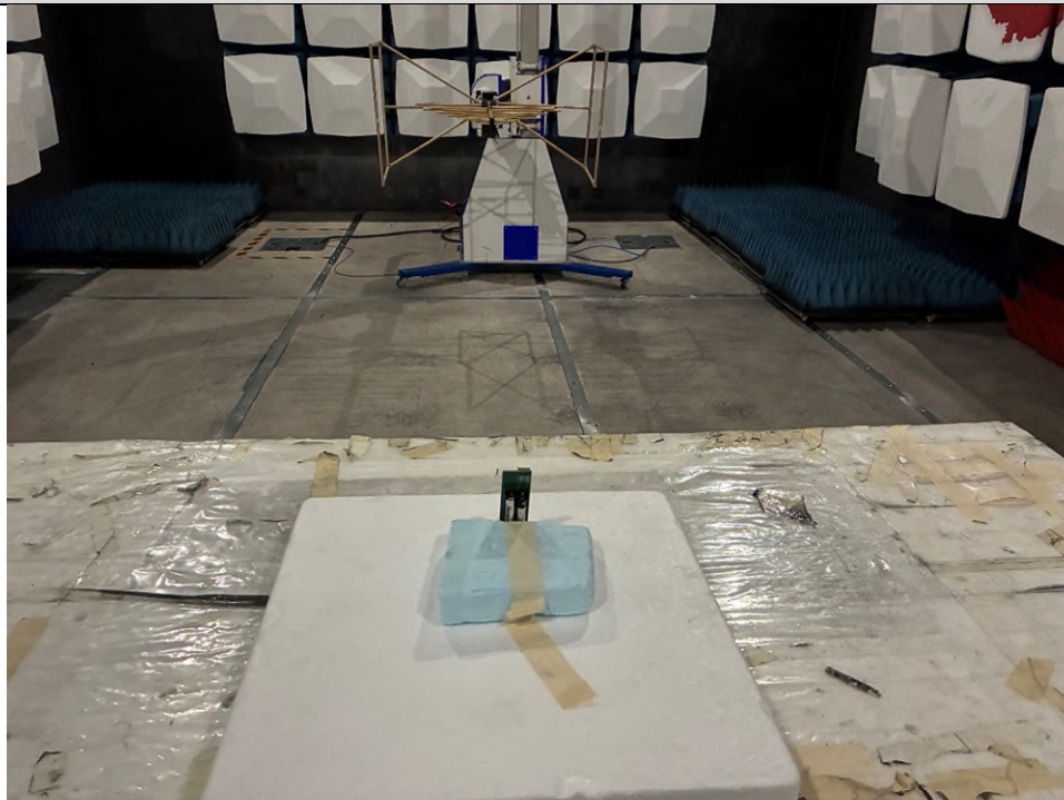
30MHz – 1GHz Rear
