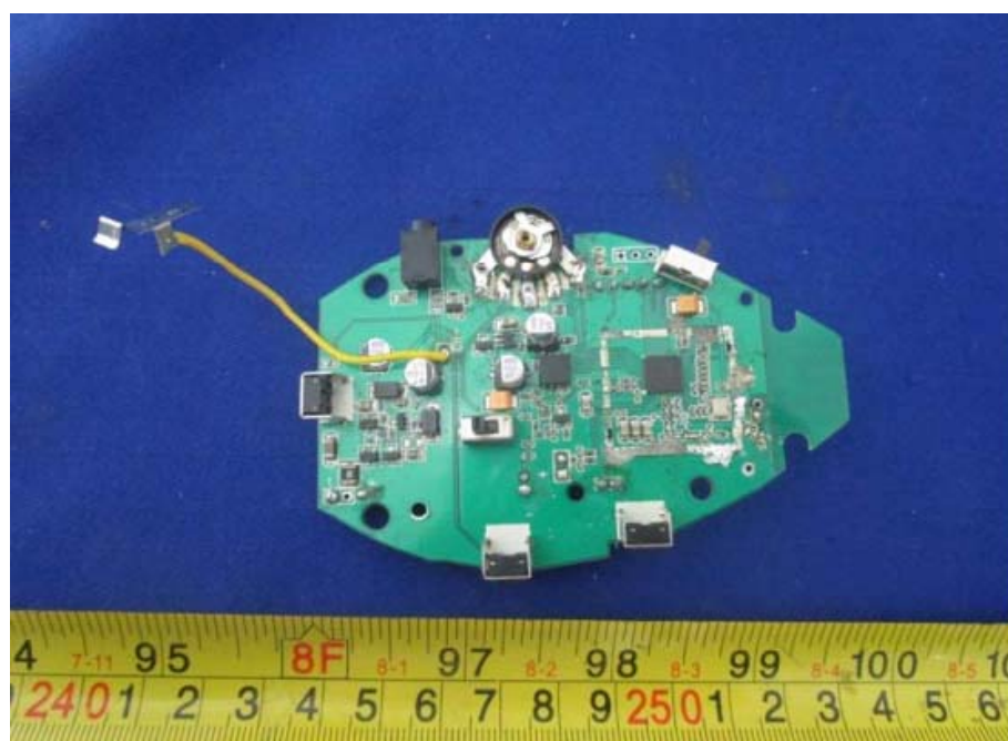
EUT – Main Board Unshield Top View
