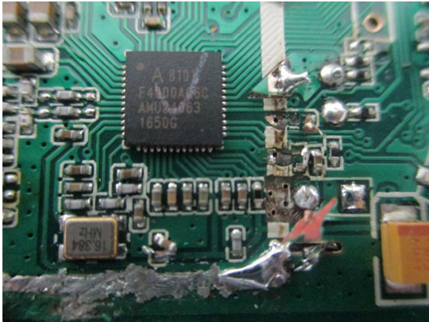
EUT – Baby Unit RF Chip View
