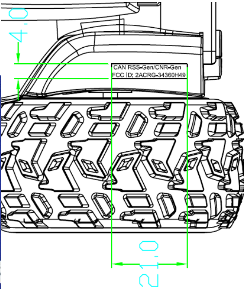
Label Size: 21mm(W) x 4mm(H)
