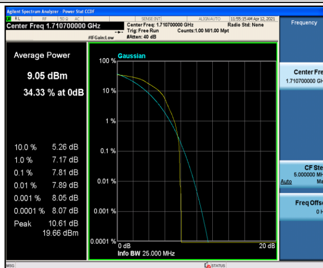
Band4-1.4MHz-16QAM-19957-1-0-Low
