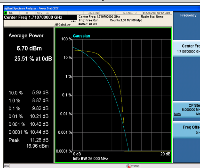
Band4-1.4MHz-16QAM-19957-6-0-Low
