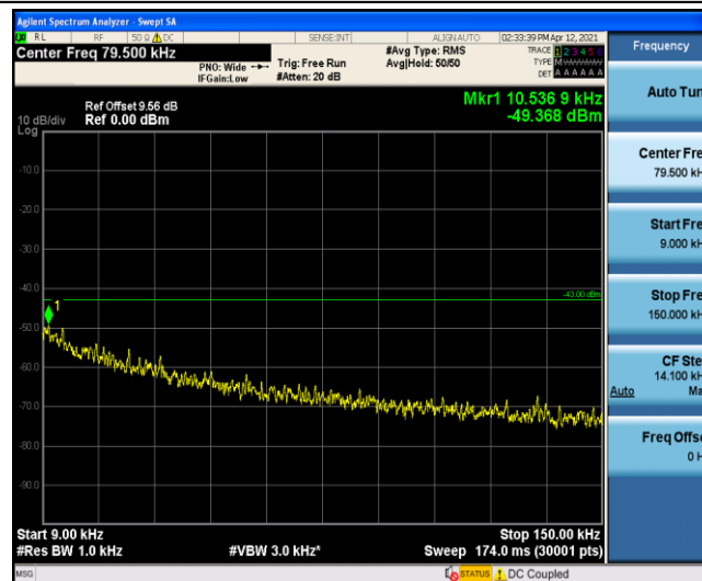
Band4-15MHz-16QAM-20325-1-0-High-0.009-0.15
