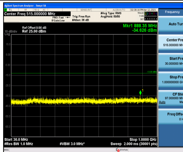
Band4-15MHz-16QAM-20175-1-0-Low-30-1000
