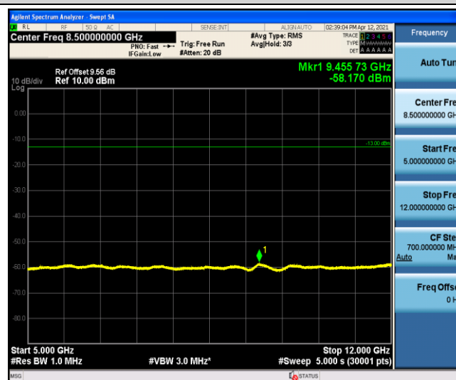
Band4-15MHz-16QAM-20175-1-0-Low-5000-12000
