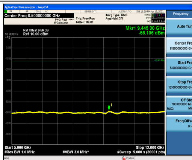
Band4-20MHz-QPSK-20050-1-0-Low-5000-12000
