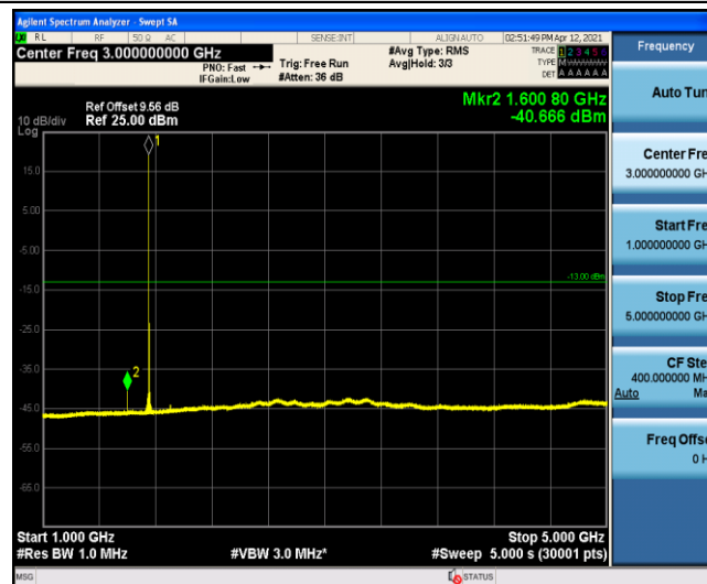
Band4-10MHz-16QAM-20350-1-0-High-1000-5000
