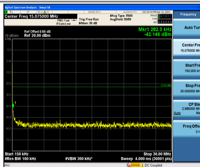
Band4-15MHz-16QAM-20325-1-0-High-0.15-30
