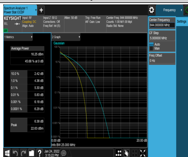
Band5-10MHz-QPSK-20600-50RB#0
