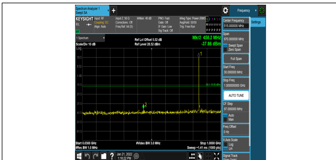
Band5-3MHz-16QAM-20635-1RB#0-Range3:30~1000MHz
