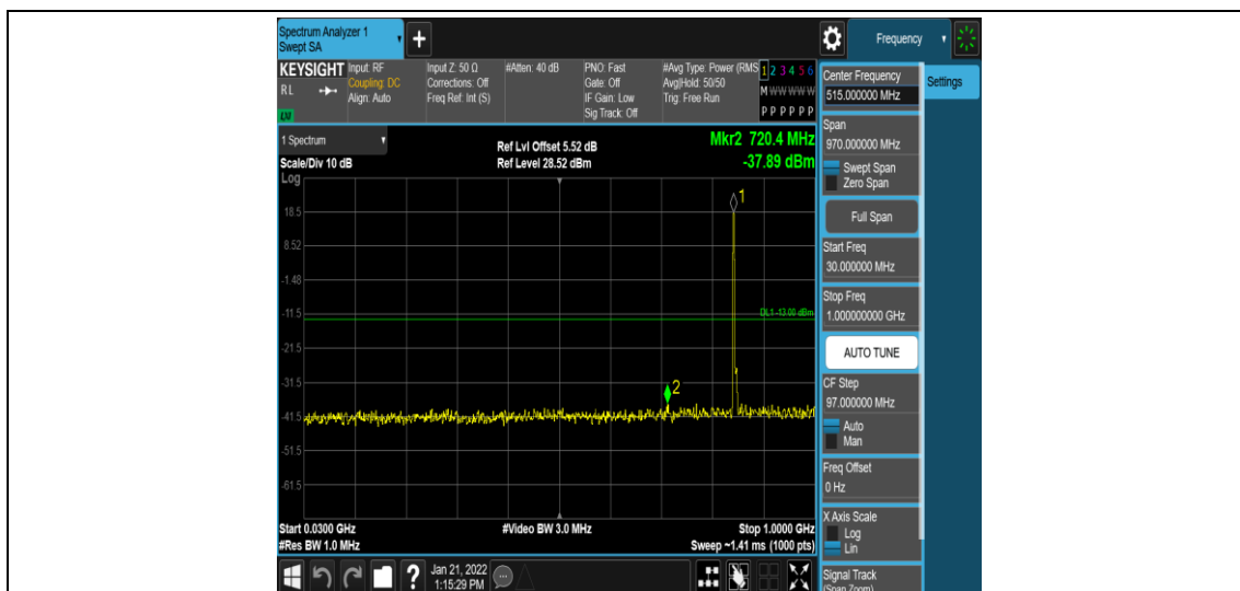
Band5-3MHz-QPSK-20635-1RB#0-Range3:30~1000MHz
