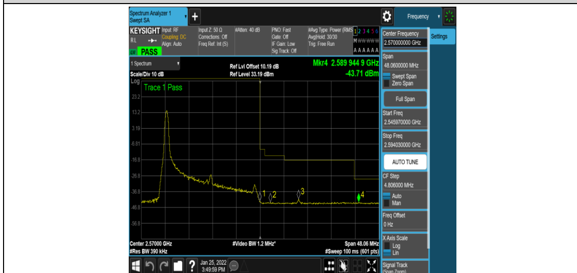
Band7-20MHz-16QAM-21350-1RB#0
