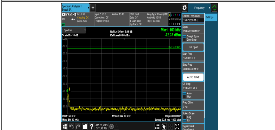
Band7-10MHz-16QAM-21100-1RB#0-Range2:0.15~30MHz
