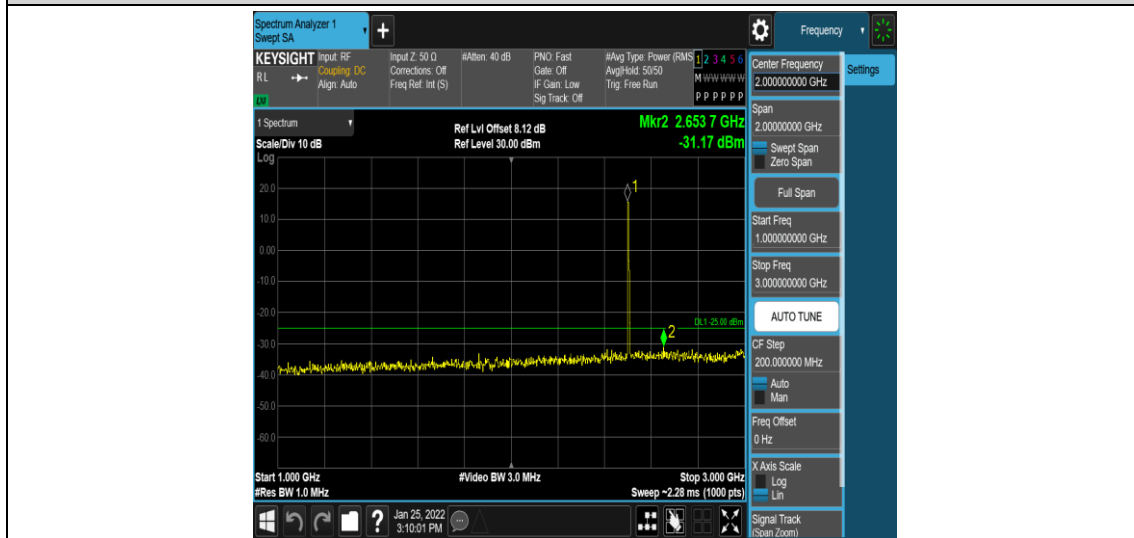
Band7-10MHz-16QAM-20800-1RB#0-Range4:1000~3000MHz
