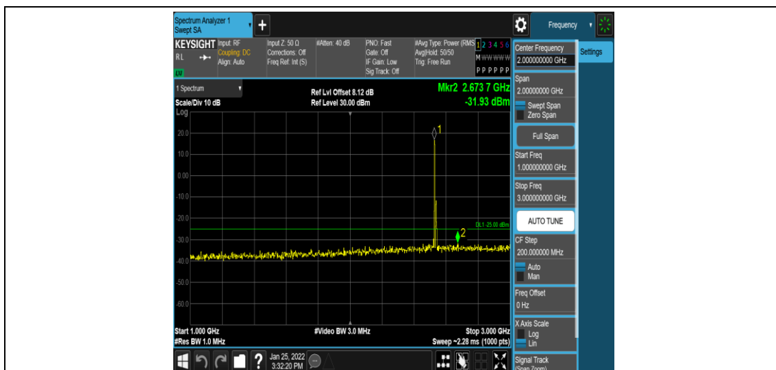
Band7-15MHz-QPSK-21100-1RB#0-Range4:1000~3000MHz
