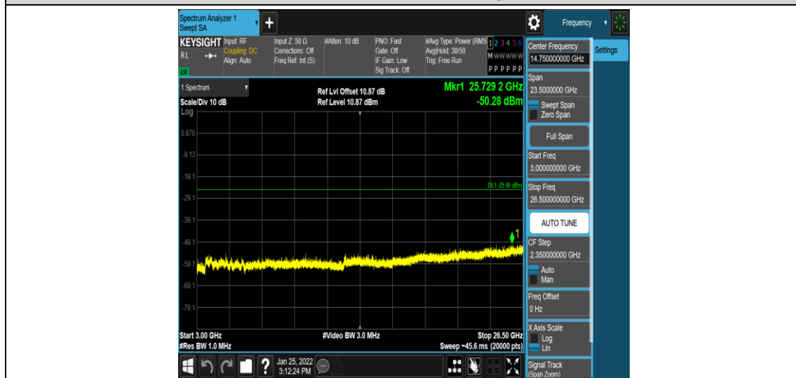
Band7-10MHz-16QAM-21100-1RB#0-Range5:3000~26500MHz
