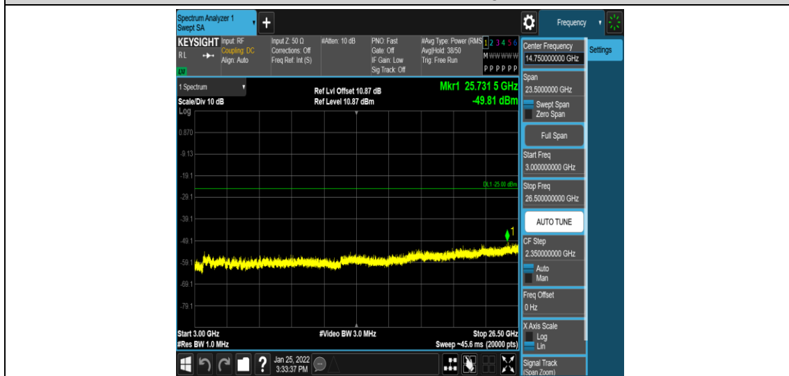
Band7-15MHz-16QAM-21100-1RB#0-Range5:3000~26500MHz
