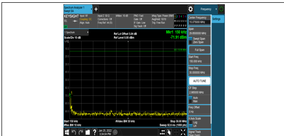
Band7-15MHz-QPSK-21375-1RB#0-Range2:0.15~30MHz
