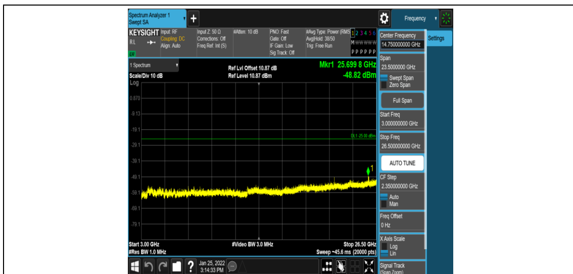
Band7-10MHz-16QAM-21400-1RB#0-Range5:3000~26500MHz
