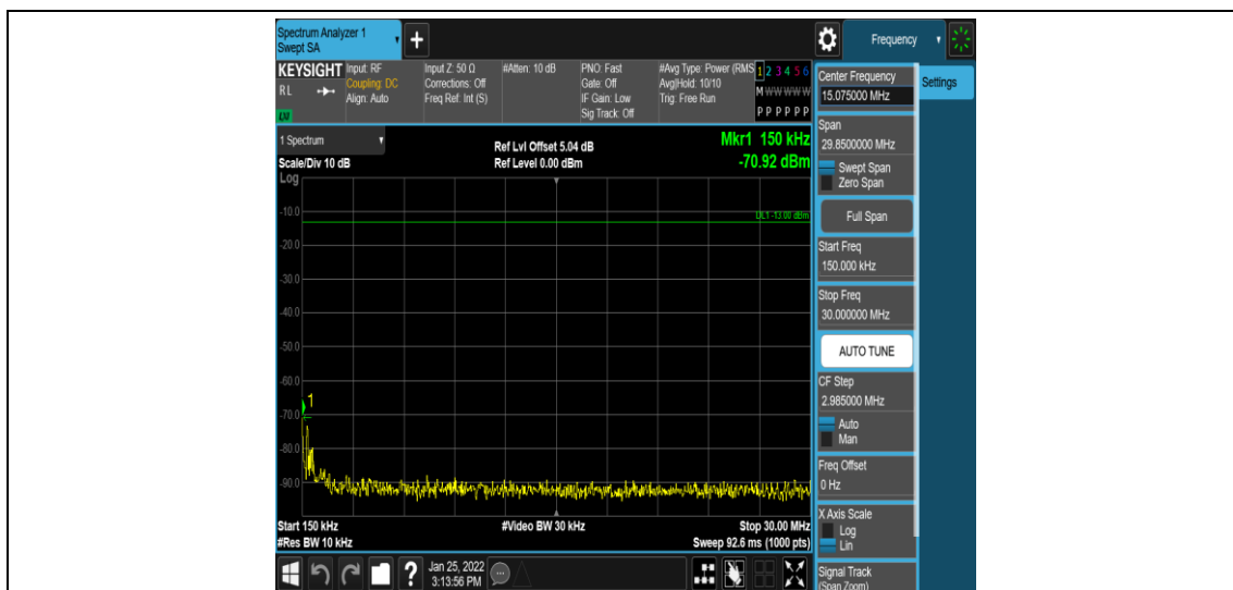
Band7-10MHz-16QAM-21400-1RB#0-Range2:0.15~30MHz
