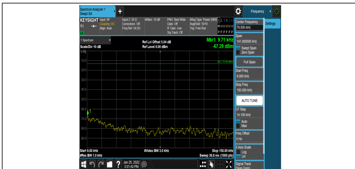
Band7-15MHz-QPSK-21100-1RB#0-Range1:0.009~0.15MHz
