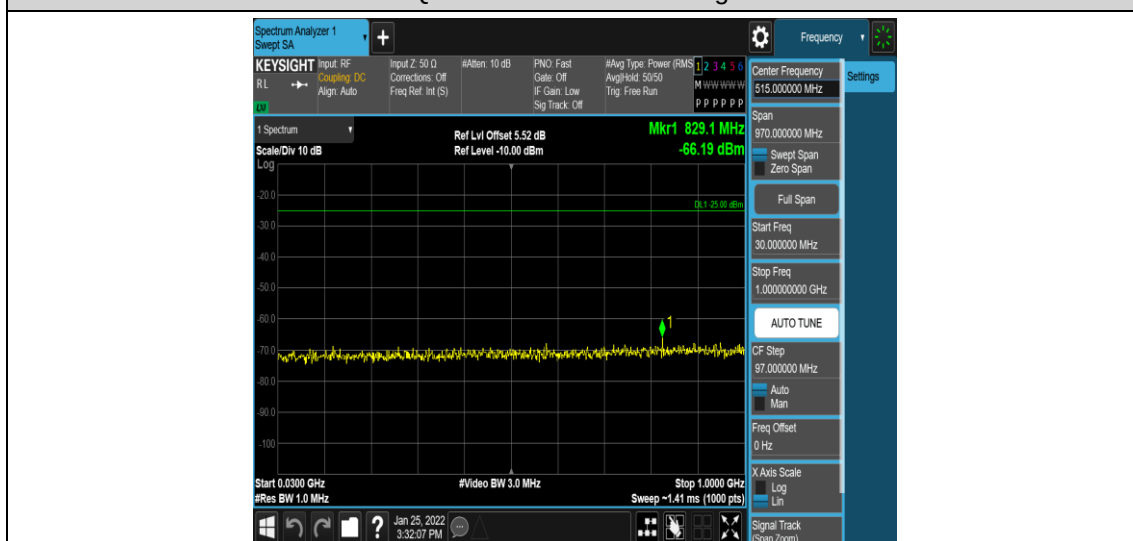
Band7-15MHz-QPSK-21100-1RB#0-Range3:30~1000MHz
