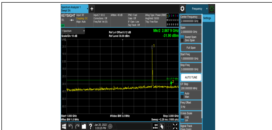
Band7-15MHz-16QAM-21100-1RB#0-Range4:1000~3000MHz
