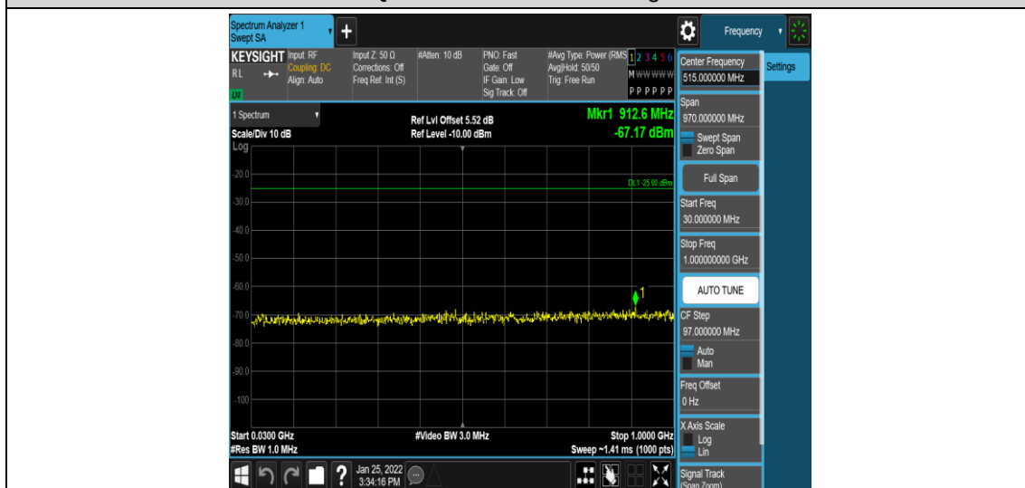
Band7-15MHz-QPSK-21375-1RB#0-Range3:30~1000MHz
