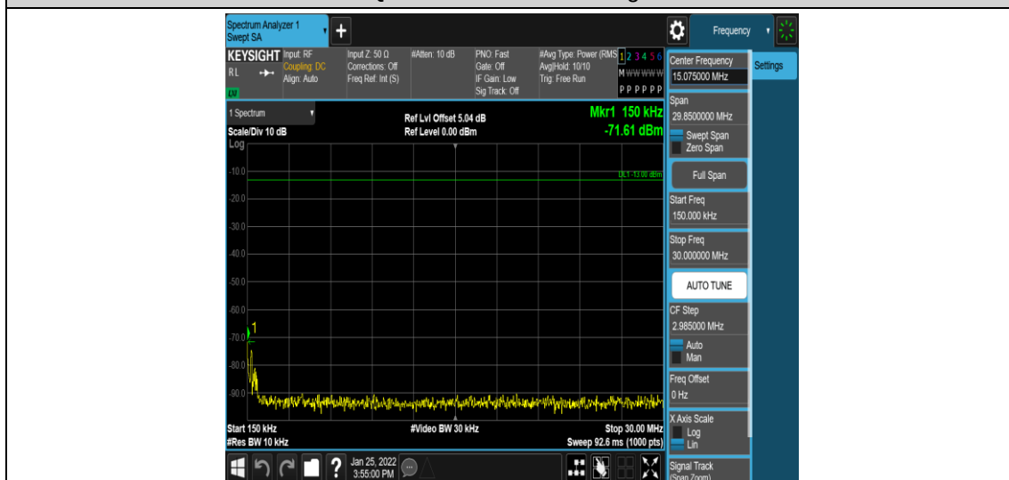
Band7-20MHz-16QAM-21100-1RB#0-Range2:0.15~30MHz
