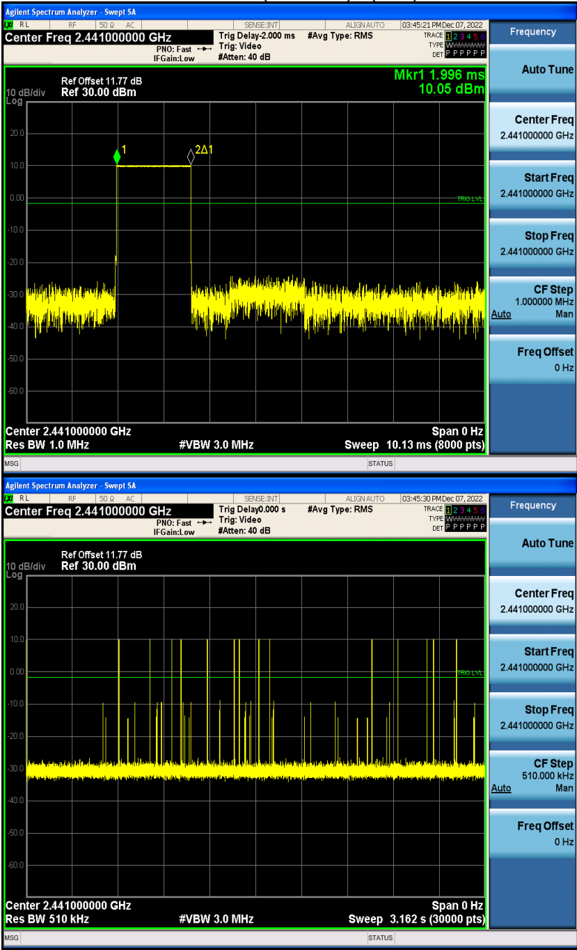
Channel 39 (2441MHz) - (DH3)
