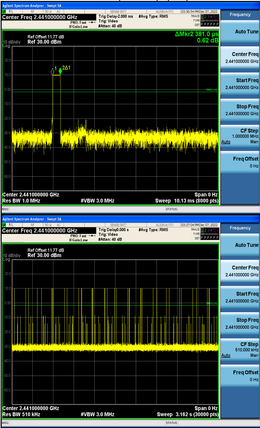
Channel 39 (2441MHz) - (DH1)
