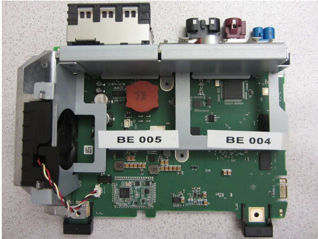
The same board also inside BEL003. Photo without shielding
