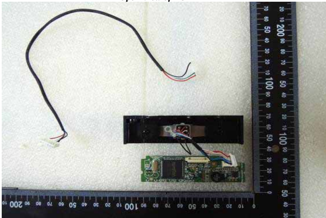
Open View of EUT – 12
