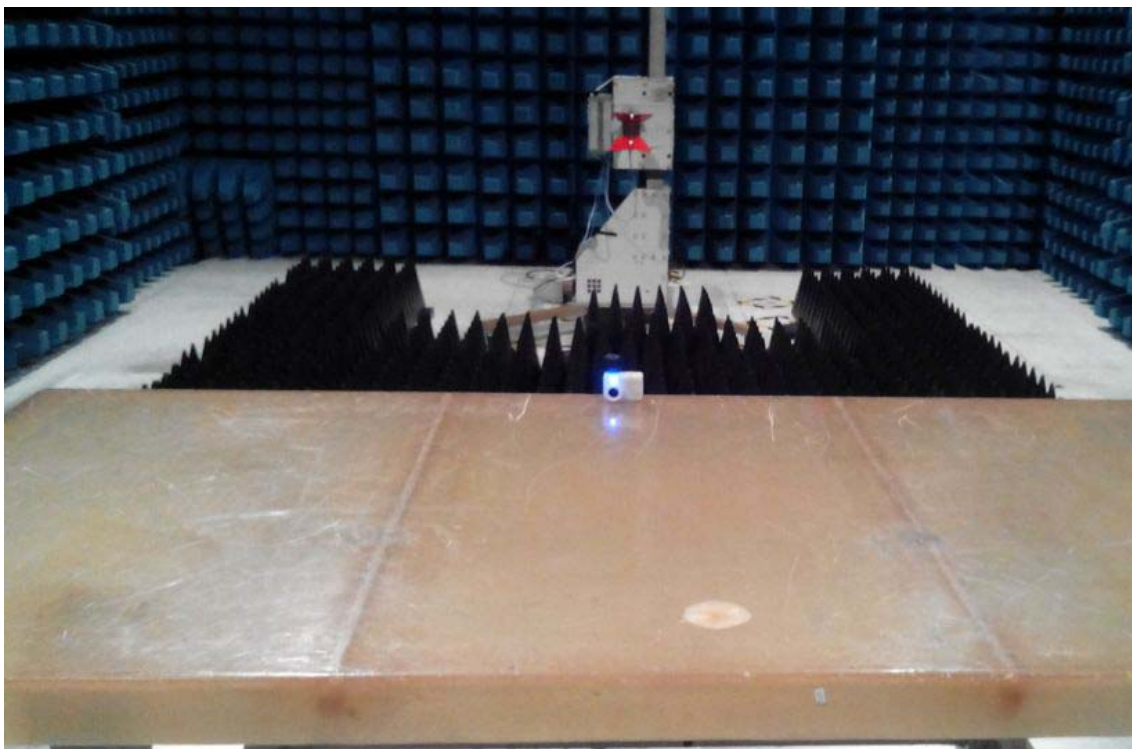
Description: Radiated Emission Test Setup for 1~18GHz
