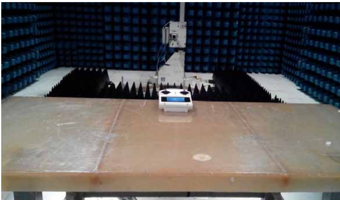
Description: Radiated Emission Test Setup for Above 18GHz
