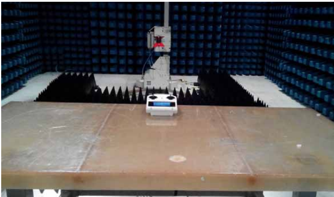
Description: Radiated Emission Test Setup for 1~18GHz
