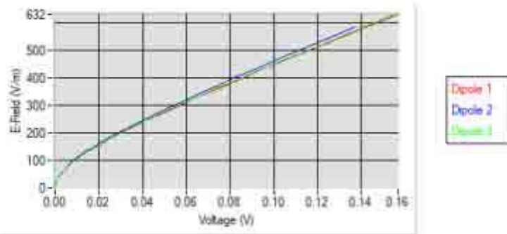
Calibration curves
