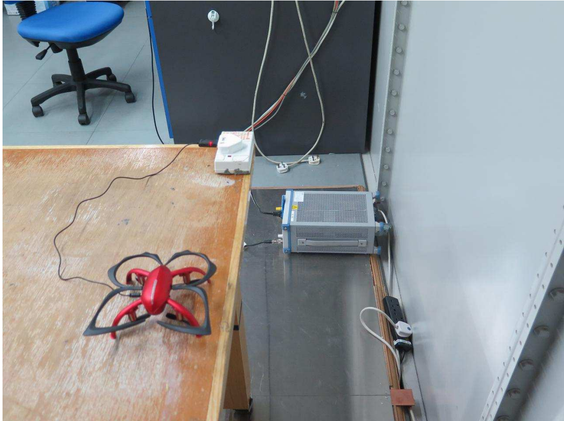
Conducted emission (Side view)
