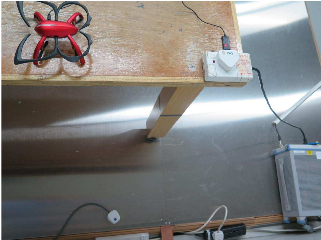
Conducted emission (Rear view)
