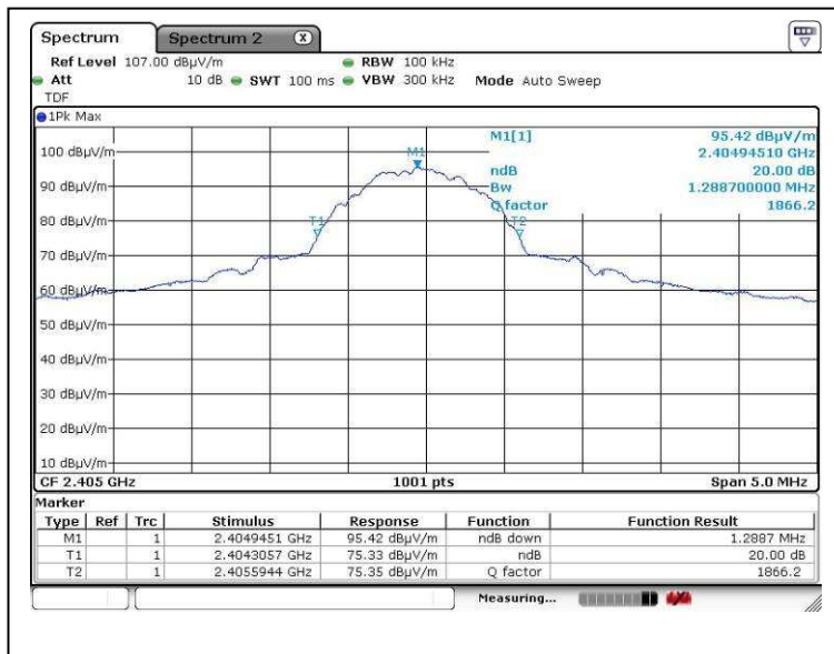
Bandwidth 1 (2405MHz)
