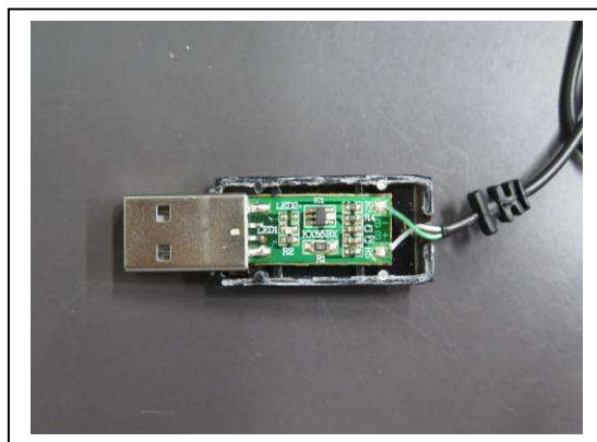
EUT antenna 2 (WiFi)
