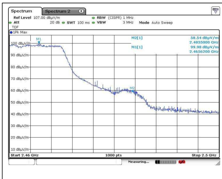
802.11g higher edge (Peak measurement)
