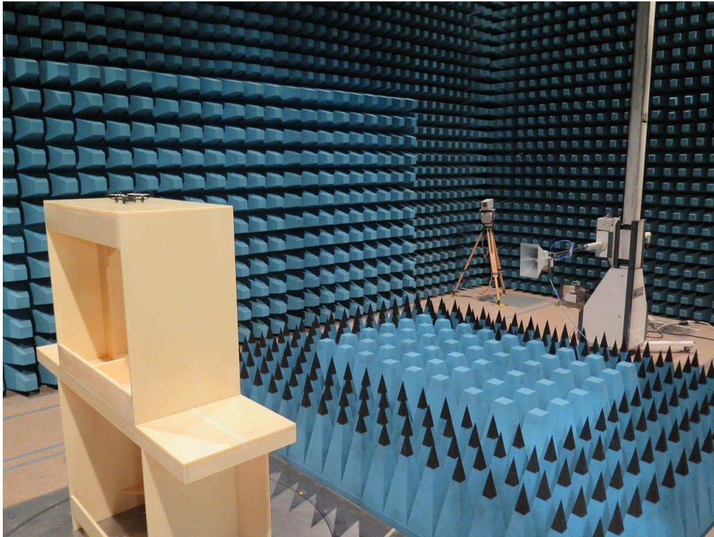
1GHz – 26GHz
