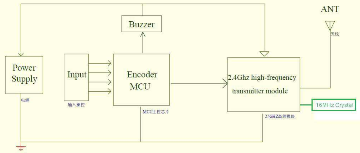
66091 TX Block Diagram
