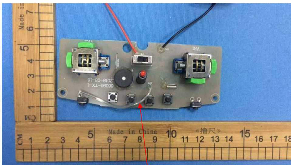
Wire Antenna
