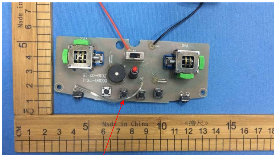
Wire Antenna
