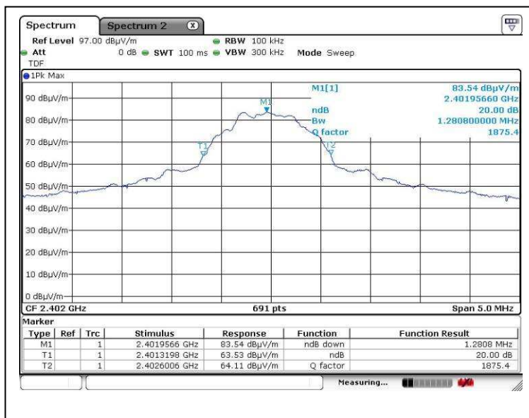
Bandwidth 1 (2402MHz)
