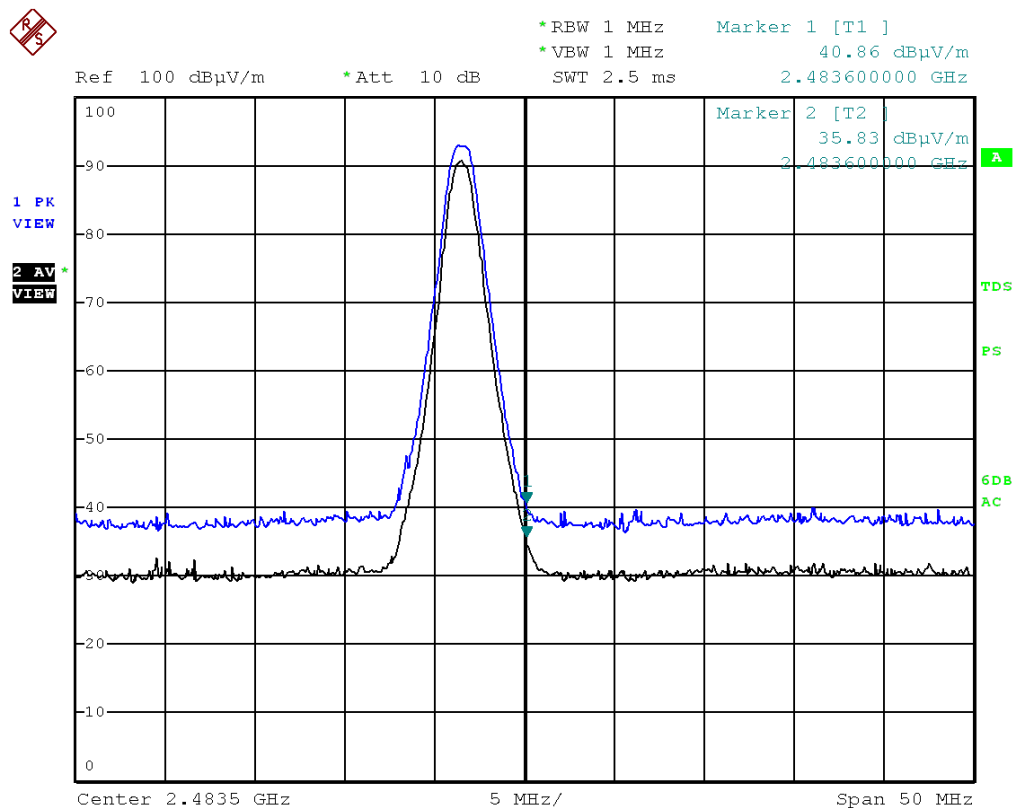
EDR(3DH5) High(Vertical)
