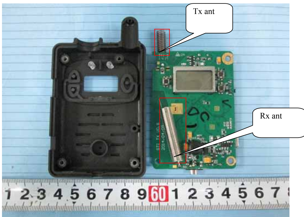
EUT-Antenna View
