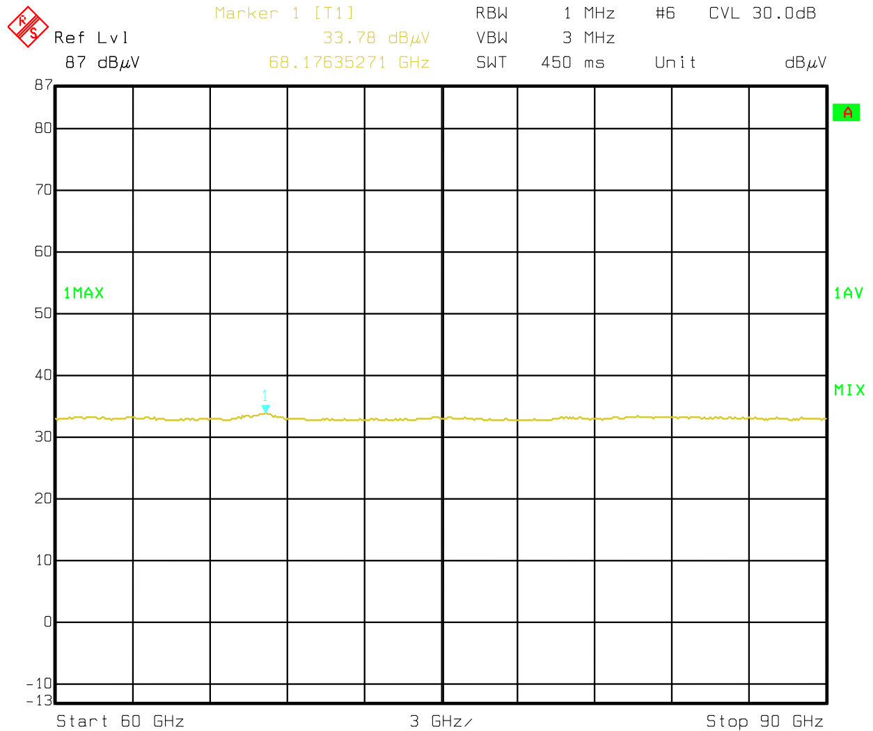
Figure 6: Spurious emission measurement results, 60GHz-90GHz, worst data(Sample 3)
