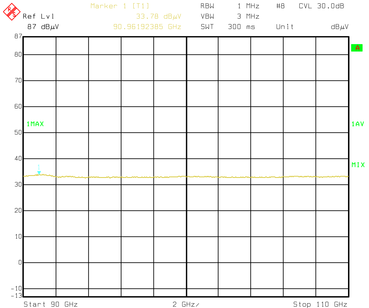
Figure 7: Spurious emission measurement results, 90GHz-110GHz, worst data(Sample 3)
