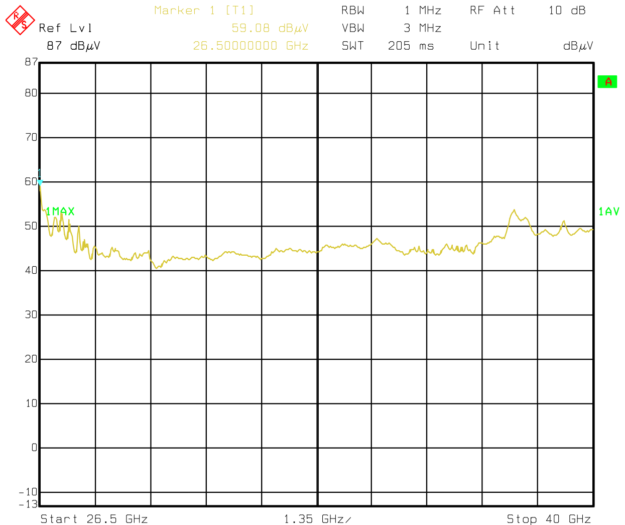
Figure 4: Spurious emission measurement results, 26.5GHz-40GHz, worst data(Sample 3)
