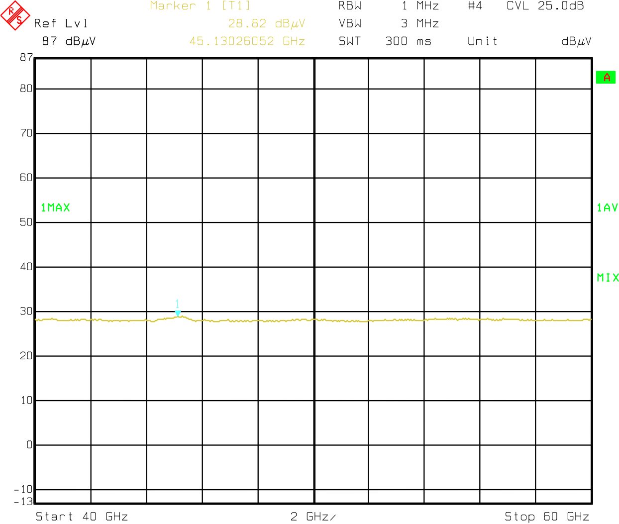
Figure 5: Spurious emission measurement results, 40GHz-60GHz, worst data(Sample 3)
