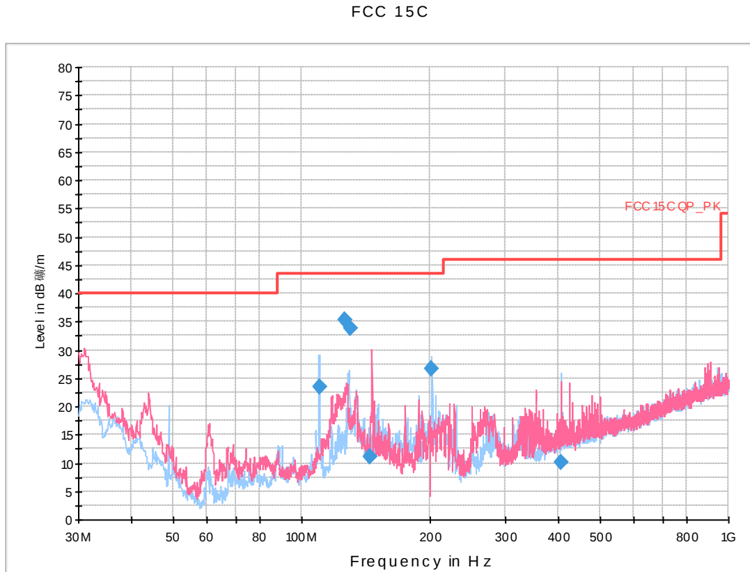
Figure 2: Radiated emission measurement results, GDRD53-PLAFDBAMAX
