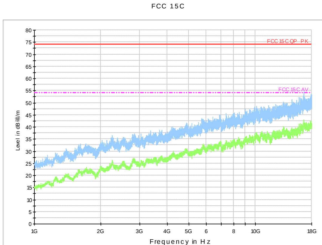
Figure 3: Radiated emission measurement results, 1GHz-18GHz, worst data(Sample 1)
