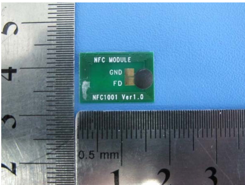
Photo 9 Appearance of PCB (NFC Module)
