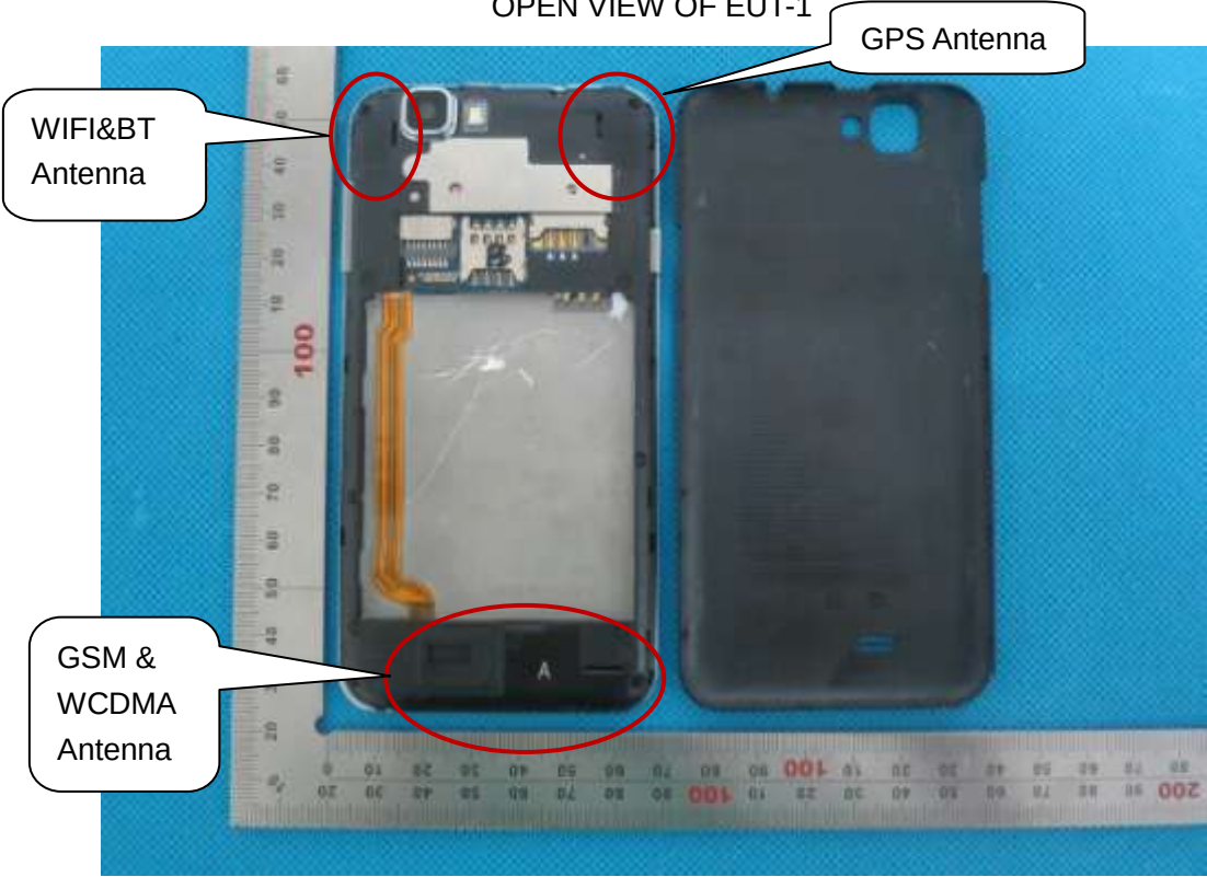
OPEN VIEW OF EUT-1
