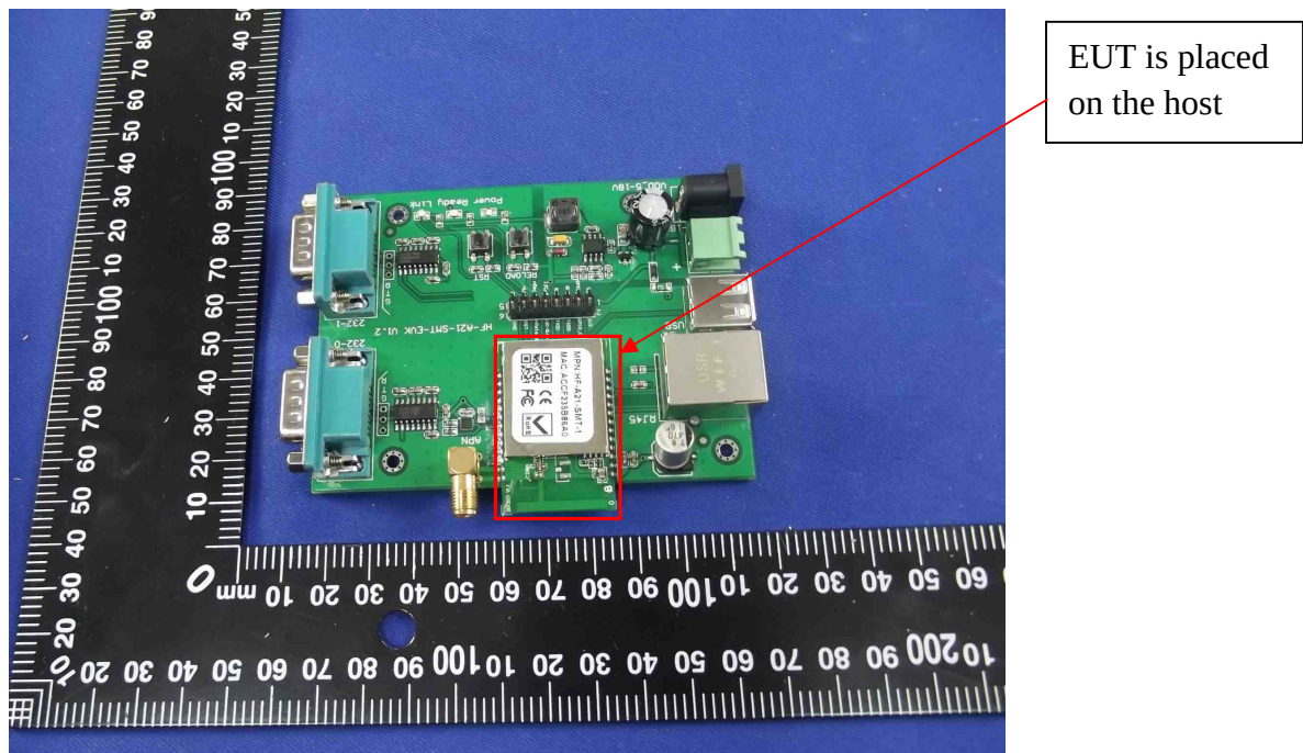
The EUT-Front View
