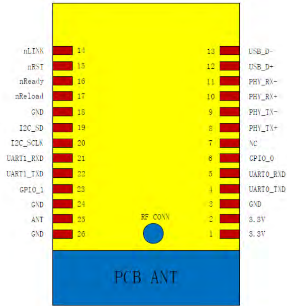
Figure 1. HF-A21-SMT Pins Map
