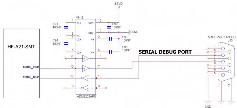
Figure 11. UART Interface Reference Design
