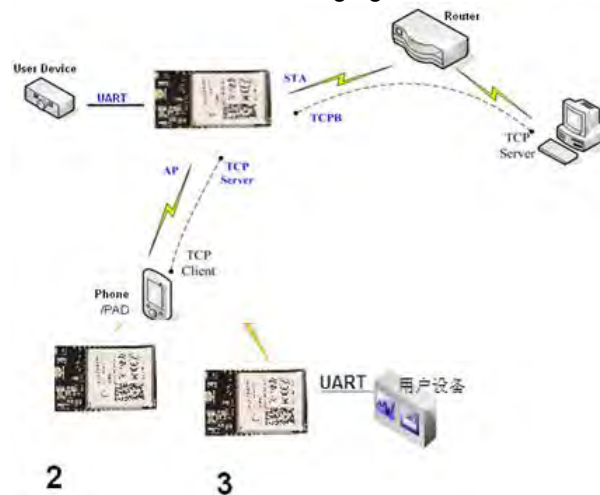
Figure 17. HF-A21-SMT AP+STA Network Structure
