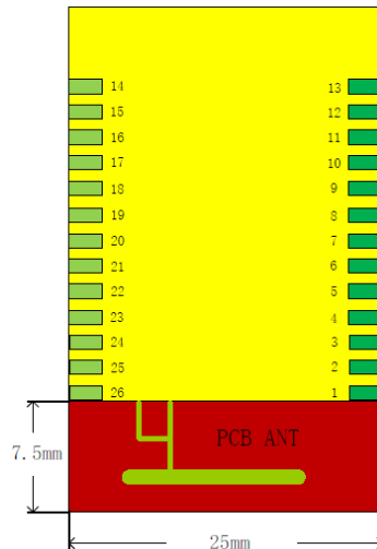
Figure 4. HF-A21-SMT Chip Antenna Keep Out Region
