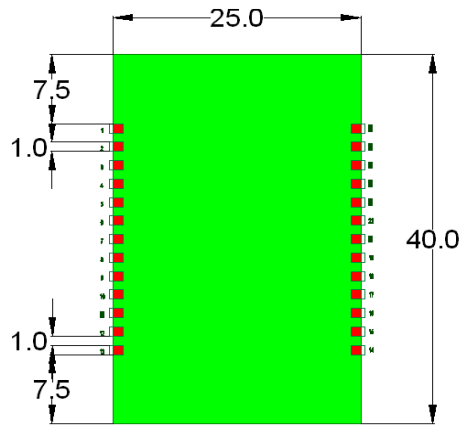
Figure 3. HF-A21-SMT Mechanical Dimension
