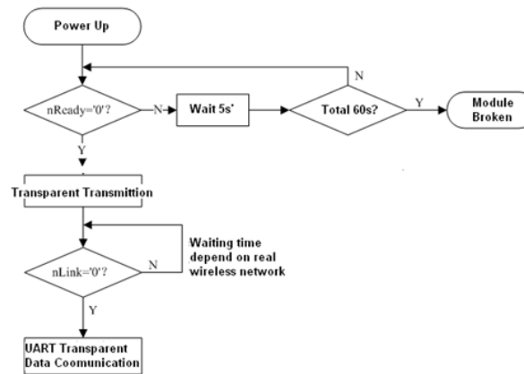
Figure 12. User MCU Software Flow Chart
