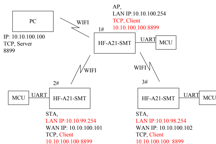
Figure 50. Wireless Data Acquisition Card Setting
