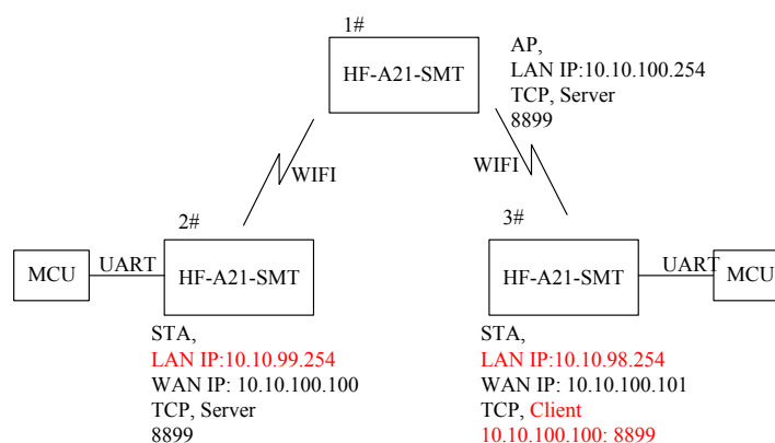
Figure 49. Two HF-A21-SMT Modules Connection Through AP
