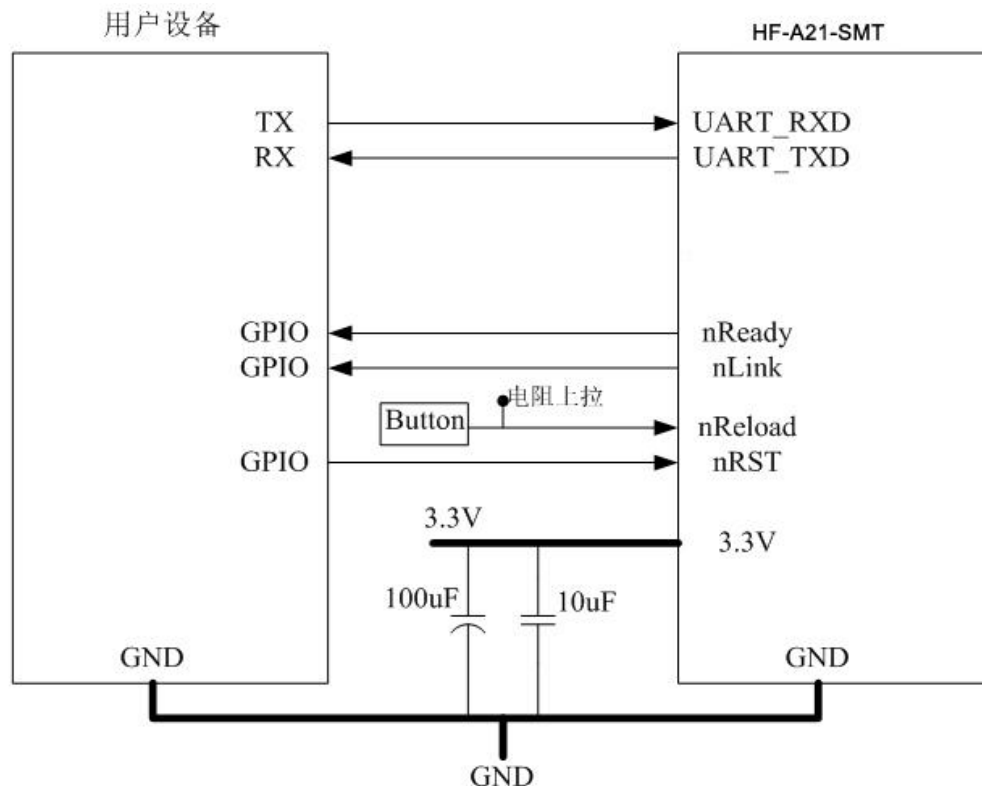
Figure 8. HF-A21-SMT Hardware Typical Application
