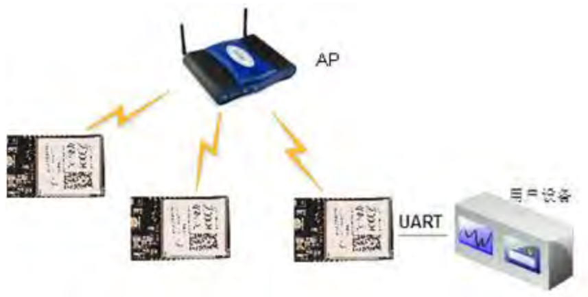
Figure 15. HF-A21-SMT Basic Wireless Network Structure
