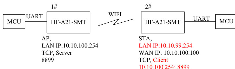
Figure 42. Configure Transparent Serial Port Connection (TCP)
