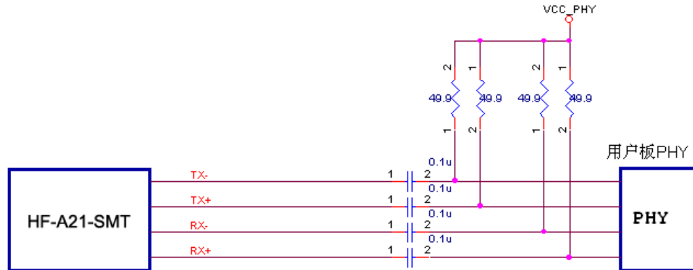
Figure 10. Ethernet Reference Design without Transformer
