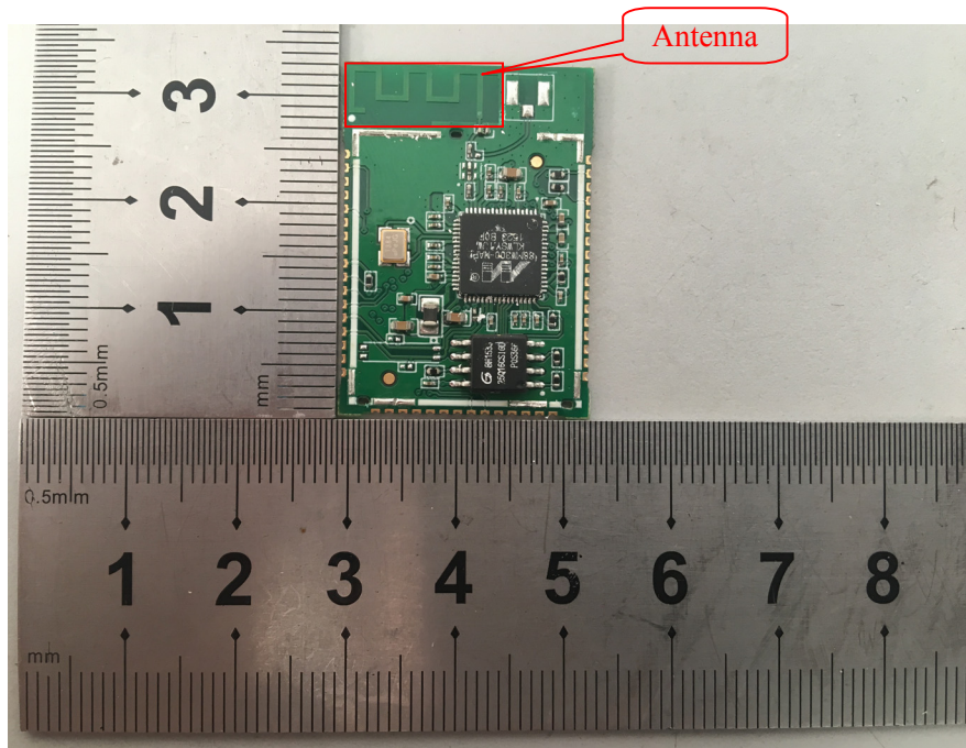
EUT – Rear View
