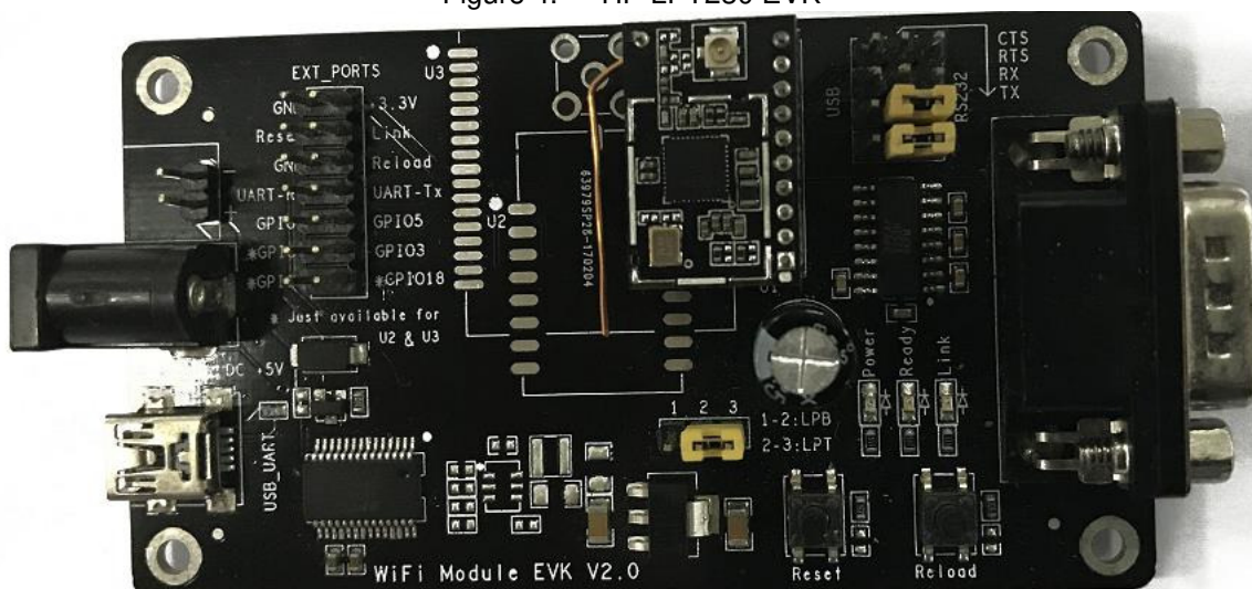
Figure 5. HF-LPT130A EVK
