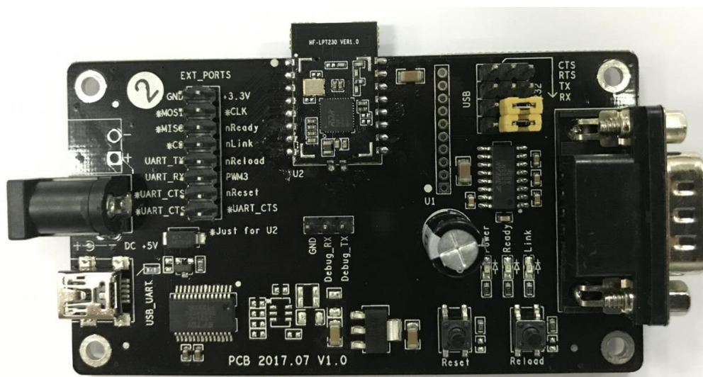
Figure 4. HF-LPT230 EVK
