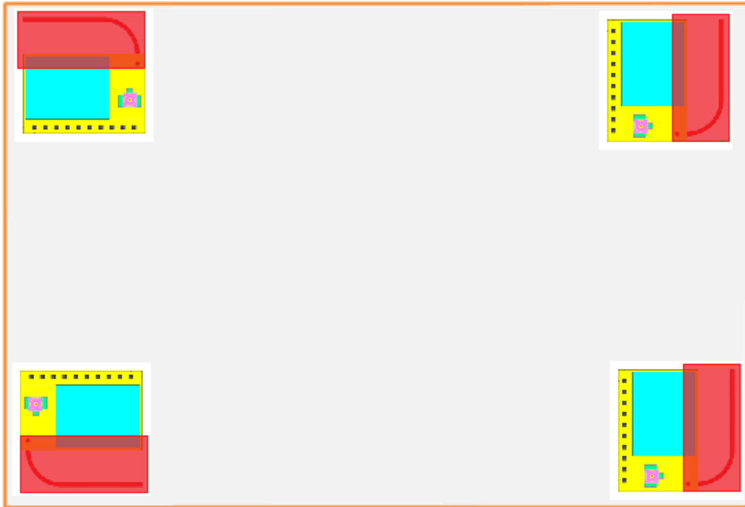
Figure 3. HF-LPT130A suggested Module Placement Region
