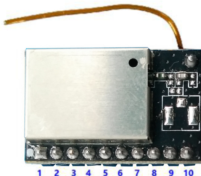
Figure 1. HF-LPT130A Pins Map
