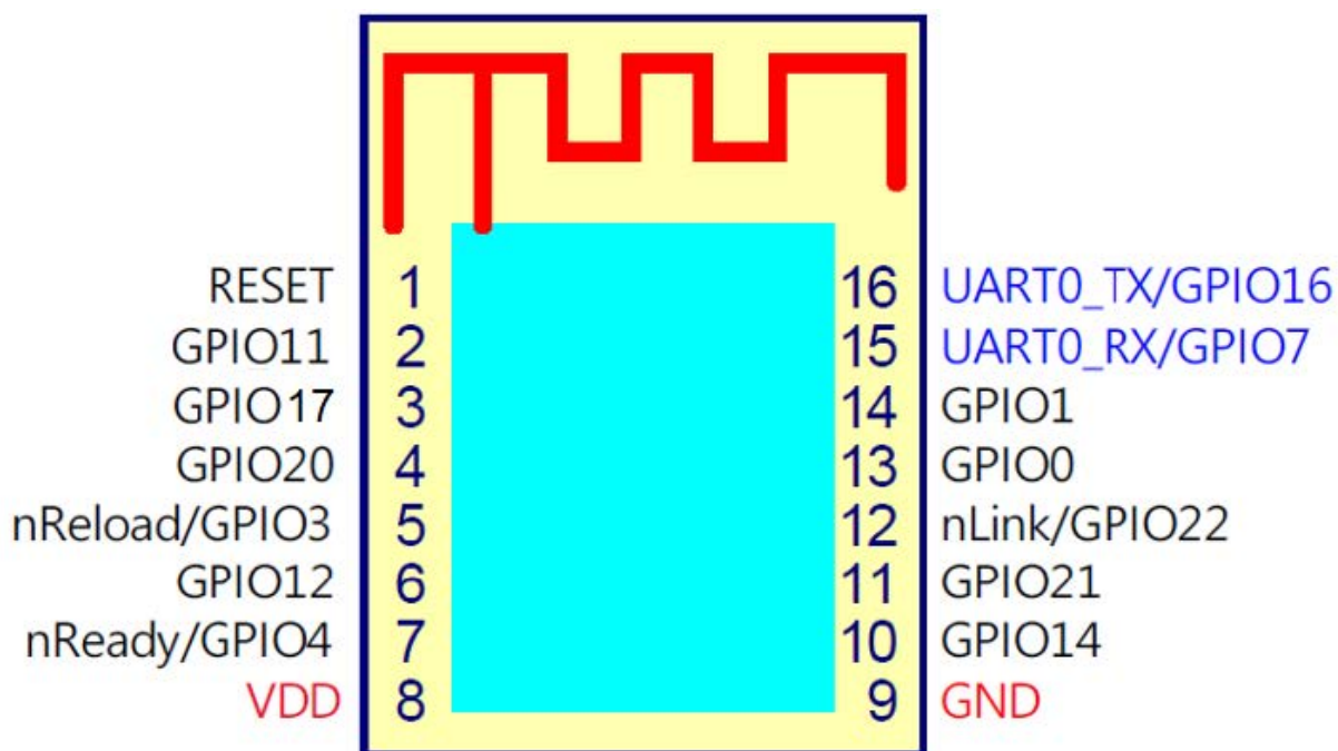
Figure 3. HF-LPT271 Pins Map
