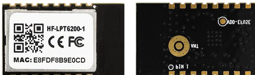
Figure 1. HF-LPT6200-1 Appearance
