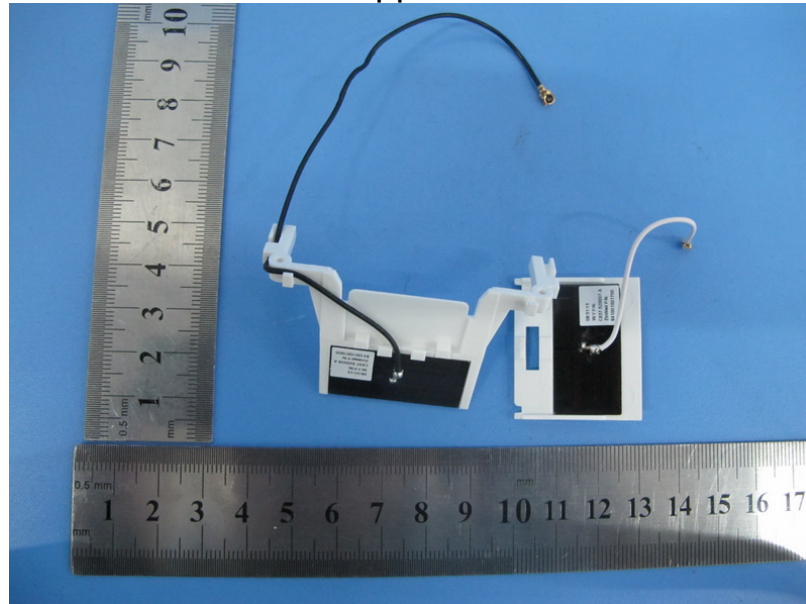
Photo 7 Appearance of Antenna
