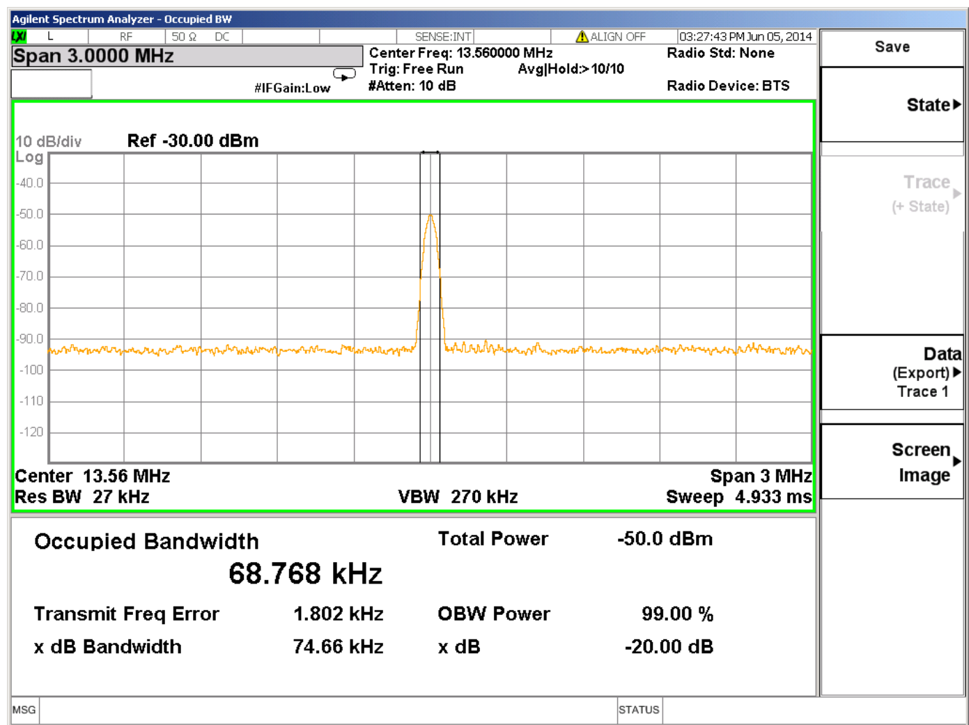
Figure 3 99% Bandwidth Graph
