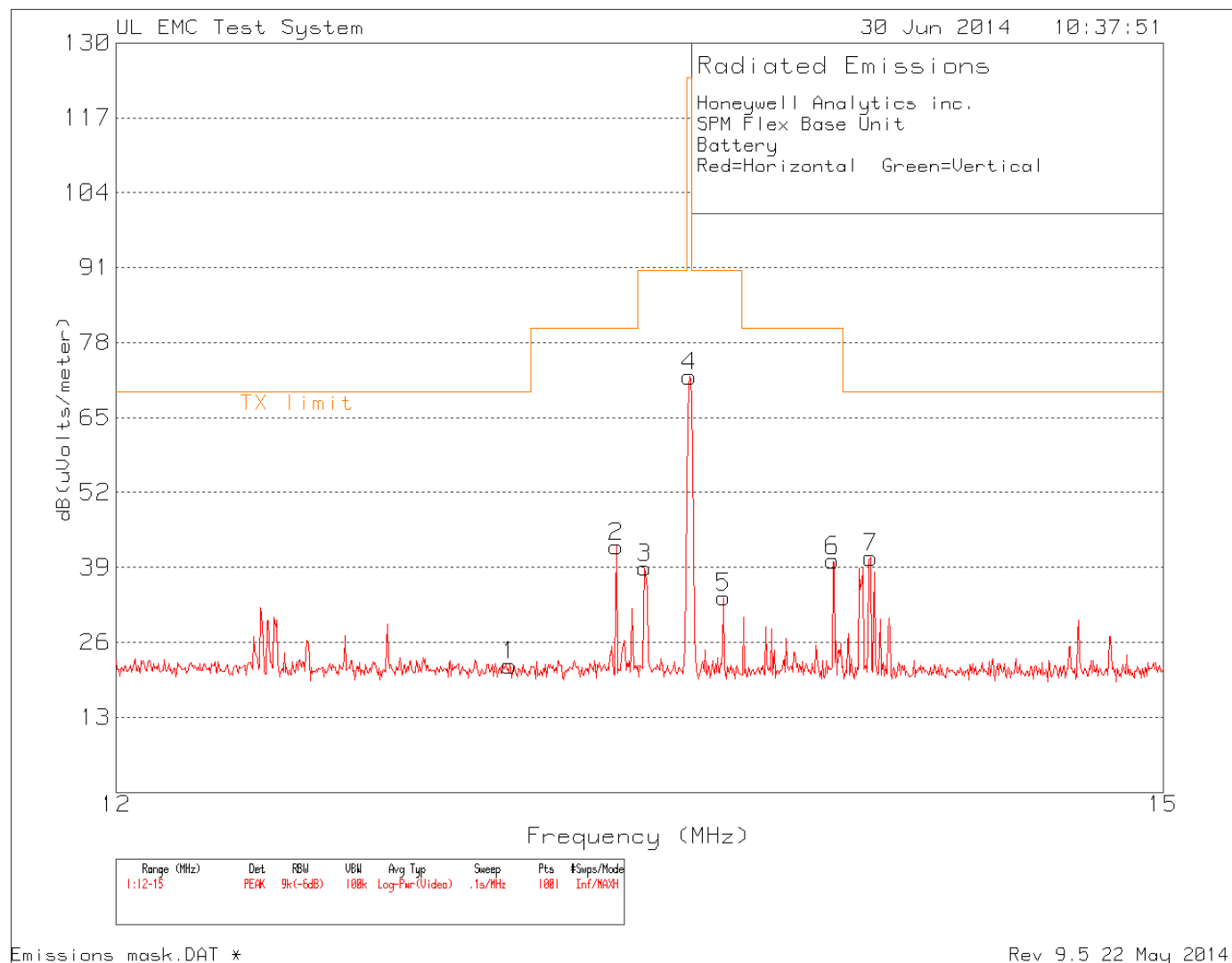
Figure 4 Radiated Emissions Graph
