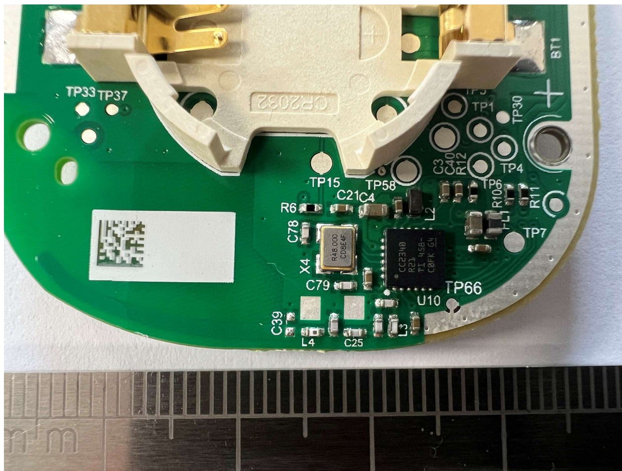
Pcba bottom view – RF module BLE IC “CC2340R21” and pcb antenna close up view
